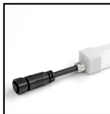
End Cap 2PIN Order Code: 7601515-06 Color: white Cable entry: front/side/bottom Picture: front
