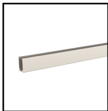
Aluminium Profile Order Code: 7601515-01 Dimension: L1000xW20.5xH17.6mm Material: aluminium Color: silver
