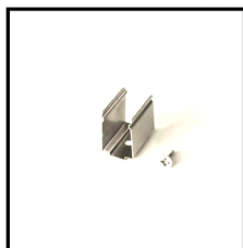
Mounting Clips Order Code: 7601515-03 Dimension: L20xW16.6xH12.4mm Material: stainless steel Color: silver Each meter led strips needs 2 clips + 2 screws
