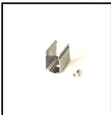
Mounting Clips Order Code: 7601020-03 Dimension: L30*W12*H22.5mm Material: stainless steel Color: silver Each meter led strips needs 2 clips + 2 screws
