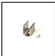
Mounting Clips Order Code: 6302020-03 Dimension: L30xW22.8xH20.9mm Material: stainless steel Color: silver Each meter led strips needs 2 clips + 2 screws
