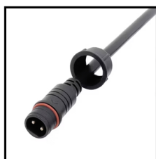
IP67 Connector 2PIN Order Code: 6302020-04 Wire gauge: 0.326mm 2 /22AWG Protection: IP67 (Mated) Connector type : Male
