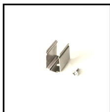
Mounting Clips Order Code: 6301515-03 Dimension: L30xW16.9xH17.8mm Material: stainless steel Color: silver Each meter led strips needs 2 clips + 2 screws
