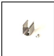
Mounting Clips Order Code: 6332020-03 Dimension: L30xW22.8xH20.9mm Material: stainless steel Color: silver Each meter led strips needs 2 clips + 2 screws
