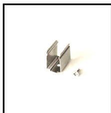
Mounting Clips Order Code: 6382020-03 Dimension: L30xW22.8xH20.9mm Material: stainless steel Color: silver Each meter led strips needs 2 clips + 2 screws
