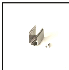
Mounting Clips Order Code: 6381515-03 Dimension: L30xW16.9xH17.8mm Material: stainless steel Color: silver Each meter led strips needs 2 clips + 2 screws
