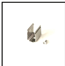
Mounting Clips Order Code: 8701616-03 Dimension: L20xW16.6xH12.4mm Material: stainless steel Color: silver Each meter led strips needs 2 clips + 2 screws
