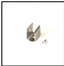
Mounting Clips Order Code: 8701616-03 Dimension: L20xW16.6xH12.4mm Material: stainless steel Color: silver Each meter led strips needs 2 clips + 2 screws
