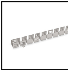
Curved Profile Order Code: 8701616-02 Dimension: L500xW17xH15mm Material: stainless steel Color: silver
