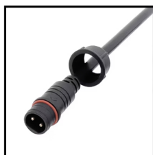
IP67 Connector 2PIN Order Code: 8701220-04 Wire gauge: 0.326mm 2 /22AWG Protection: IP67 (Mated) Connector type : Male
