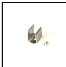
Mounting Clips Order Code: 8701220-03 Dimension: L30*W14*H22.5mm Material: stainless steel Color: silver Each meter led strips needs 2 clips + 2 screws
