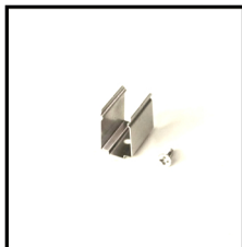
Mounting Clips Order Code: 8701020-03 Dimension: L30*W12*H22.5mm Material: stainless steel Color: silver Each meter led strips needs 2 clips + 2 screws
