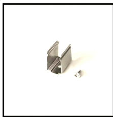
Mounting Clips Order Code: 8701010-03 Dimension: L11.6xW8xH7.6mm Material: stainless steel Color: silver Each meter led strips needs 2 clips + 2 screws
