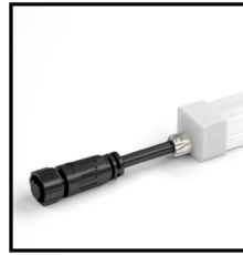
End Cap 2PIN Order Code: 8701010-06 Color: white Cable entry: front/side/bottom Picture: front
