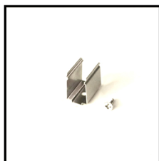
Mounting Clips Order Code: 8700714-03 Dimension: L20*W7.9*H13.6mm Material: stainless steel Color: silver Each meter led strips needs 2 clips + 2 screws
