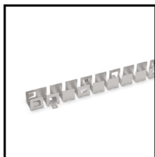
Curved Profile Order Code: 8700714-02 Dimension: L1000*W7*H12mm Material: stainless steel Color: silver
