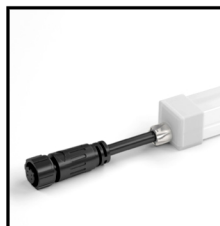
End Cap 2PIN Order Code: 8700714-06 Color: white Cable entry: front/side/bottom Picture: front
