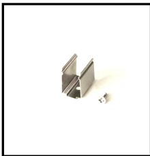
Mounting Clips Order Code: 8730614-03 Dimension: L20*W7.9*H13.6mm Material: stainless steel Color: silver Each meter led strips needs 2 clips + 2 screws
