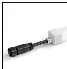
End Cap 5PIN Order Code: 8761515-06 Color: white Cable entry: front/side/bottom Picture: front
