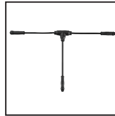
IP67 T Type Connector Order Code : 8761220-08 Wire Gauge : 0.326mm 2 /22AWG Protection : IP67 (Mated)
