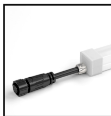
End Cap 5PIN Order Code: 8761020-06 Color: white Cable entry: front/side/bottom Picture: front
