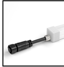
End Cap 3PIN Order Code: 8771520-06 Color: white Cable entry: front/side/bottom Picture: front
