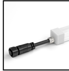
End Cap 3PIN Order Code: 8771220-06 Color: white Cable entry: front/side/bottom Picture: front
