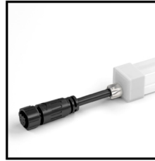
End Cap 3PIN Order Code: 8770816-06 Color: white Cable entry: front/side/bottom Picture: front
