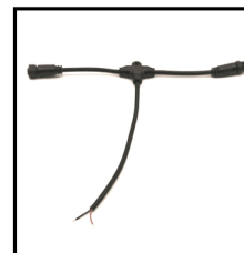
IP67 T Type Connector Order Code: 8751220-08 Wire Gauge: 0.326mm 2 /22AWG Protection: IP67 (Mated)
