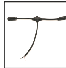
IP67 T Type Connector Order Code: 8750816-08 Wire Gauge: 0.326mm 2 /22AWG Protection: IP67 (Mated)
