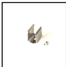
Mounting Clips Order Code: 8781520-03 Dimension: L30*W15*H20mm Material: stainless steel Color: silver Each meter led strips needs 2 clips + 2 screws
