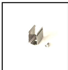
Mounting Clips Order Code: 8781515-03 Dimension: L20xW16.6xH12.4mm Material: stainless steel Color: silver Each meter led strips needs 2 clips + 2 screws
