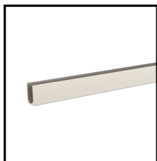
Aluminium Profile Order Code: 8781220-01 Dimension: L1000*W14*H22.5mm Material: aluminium Color: silver
