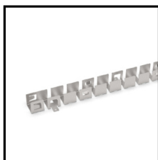
Curved Profile Order Code: 8781020-02 Dimension: L1000*W12.4*H22.6mm Material: stainless steel Color: silver
