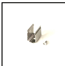
Mounting Clips Order Code: 8781020-03 Dimension: L30*W12*H22.5mm Material: stainless steel Color: silver Each meter led strips needs 2 clips + 2 screws
