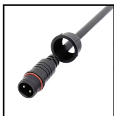
IP67 Connector 2PIN Order Code: 8781020-04 Wire gauge: 0.326mm 2 /22AWG Protection: IP67 (Mated)
