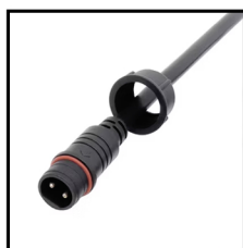
IP67 Connector 2PIN Order Code: 8780816-04 Wire gauge: 0.326mm 2 /22AWG Protection: IP67 (Mated)
