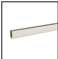
Aluminium Profile Order Code: 8780816-01 Dimension: L1000*W10*H17mm Material: aluminium Color: silver
