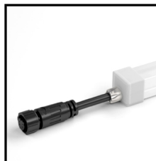
End Cap 2PIN Order Code: 8780816-06 Color: white Cable entry: front/side/bottom Picture: front
