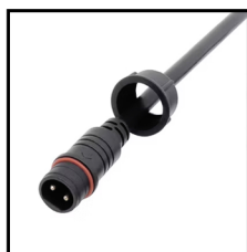
IP67 Connector 2PIN Order Code: 8780714-04 Wire gauge: 0.326mm 2 /22AWG Protection: IP67 (Mated)
