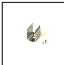
Mounting Clips Order Code: 8780714-03 Dimension: L20*W7.9*H13.6mm Material: stainless steel Color: silver Each meter led strips needs 2 clips + 2 screws
