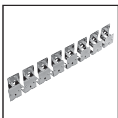
Curved Profile Order Code : 8791520-02 Dimension : L1020*W15*H20 Material : stainless steel Color : silver
