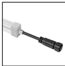
End Cap 5PIN Order Code : 8791515-06 Color : white Cable entry : front/side/bottom Picture : front
