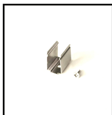
Mounting Clips Order Code: 7701515-03 Dimension: L20xW16.6xH12.4mm Material: stainless steel Color: silver Each meter led strips needs 2 clips + 2 screws
