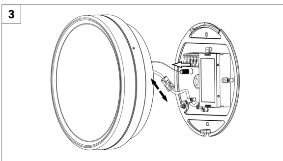
Disconnect the wires and safety steel rope
