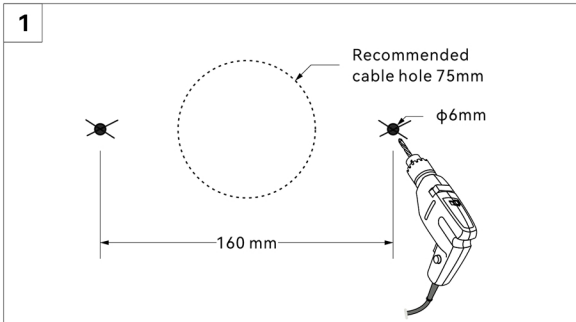
Dimensions of mounting holes
