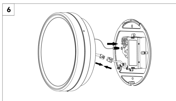
Connect the safety steel rope and wires.
