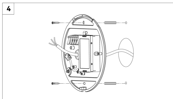
Put AC cable through the hole, and fix the backplate to the wall by 2 screws
