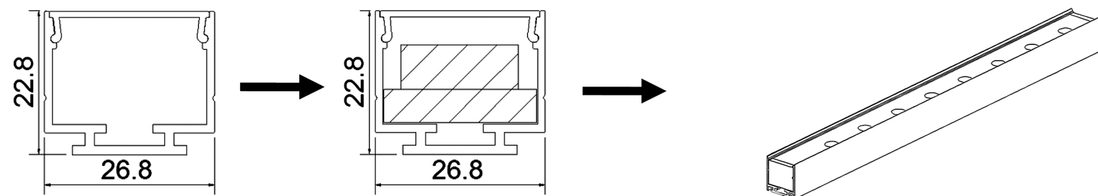
Alu profile with PC cover : 7022205-03
