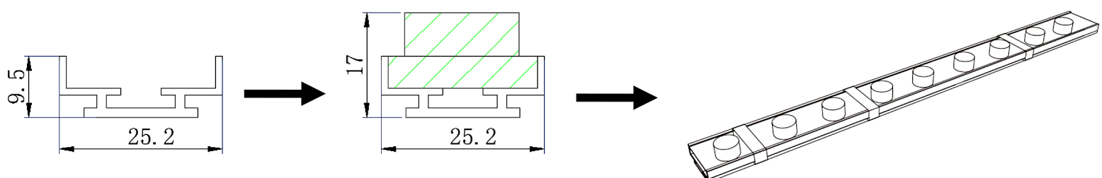
Alu Profile installation : 7022205-02
