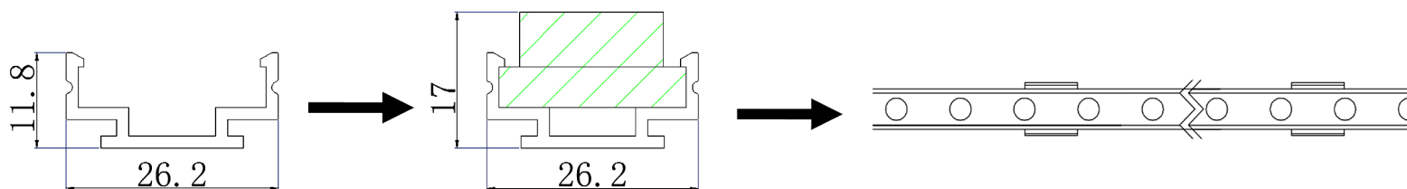
Clips installation : 7022205-01
