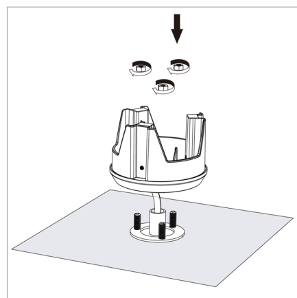
6. Fix the mounting plate to the J Anchor Bolt Kit
