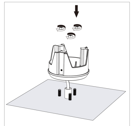
6. Fix the mounting plate
