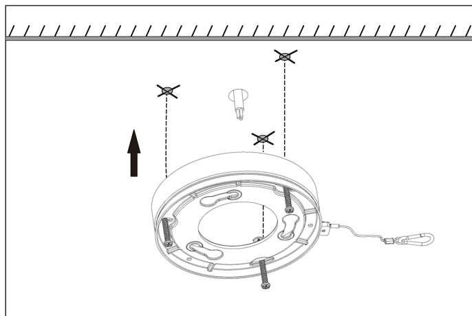
3. Fix the base to the ceiling with self-tapping screws.
