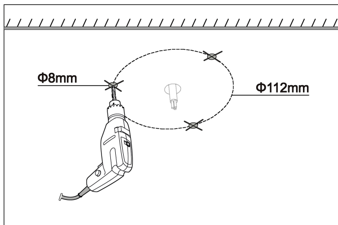
1. Punch three holes (size: \Phi 8\text{mm} \times 50\text{mm} ) at the position of three equal parts on a circle (diameter : 112\text{mm} ) in the ceiling.
