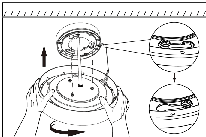
5. Align the hole, and screw the lamp body clockwise into the base (about 30^\circ ). If there is a slight looseness, it indicates that it is rotated in place.
