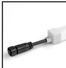
End Cap 2PIN Order Code: 8901818-06 Color: white Cable entry: front/side/bottom Picture: front
