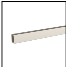
Aluminium Profile Order Code: 8901818-01 Dimension: L1000xW19.8H16.9 Material: aluminium Color: silver
