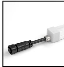
End Cap 2PIN Order Code: 8901010-06 Color: white Cable entry: front/side/bottom Picture: front
