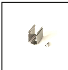
Mounting Clips Order Code: 8901010-05 Dimension: L11.6xW8xH7.6mm Material: stainless steel Color: silver Each meter led strips needs 2 clips + 2 screws
