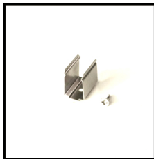
Mounting Clips Order Code: 8931818-03 Dimension: L30xW19.8H16.9 Material: stainless steel Color: silver Each meter led strips needs 2 clips + 2 screws
