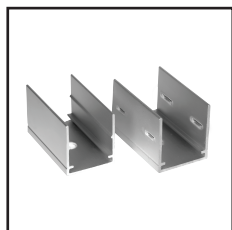
Mounting Clips Order Code : 8911616-03 Dimension : L20xW16.6xH12.4mm Material : stainless steel Color : silver Each meter led strips needs 2 clips + 2 screws
