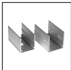
Mounting Clips Order Code : 8921616-03 Dimension : L20xW16.6xH12.4mm Material : stainless steel Color : silver Each meter led strips needs 2 clips + 2 screws
