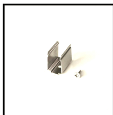
Mounting Clips Order Code: 8921010-03 Dimension: L11.6xW8xH7.6mm Material: stainless steel Color: silver Each meter led strips needs 2 clips + 2 screws
