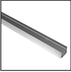
Aluminium Profile Order Code : 8961616-01 Dimension : L1000xW18xH18mm Material : aluminium Color : silver
