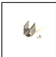
Mounting Clips Order Code: 8961515-03 Dimension: L20xW16.6xH12.4mm Material: stainless steel Color: silver Each meter led strips needs 2 clips + 2 screws
