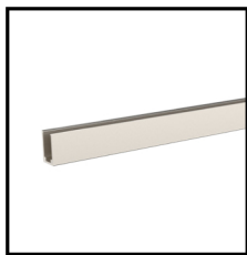
Aluminium Profile Order Code: 8961010-01 Dimension: L1000xW13xH12.4mm Material: aluminium Color: silver
