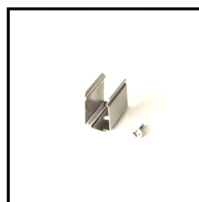
Mounting Clips Order Code: 8961818-03 Dimension: L30xW19.8H16.9 Material: stainless steel Color: silver Each meter led strips needs 2 clips + 2 screws
