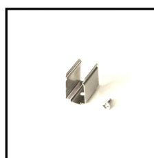
Mounting Clips Order Code: 8921818-03 Dimension: L30xW19.8H16.9 Material: stainless steel Color: silver Each meter led strips needs 2 clips + 2 screws
