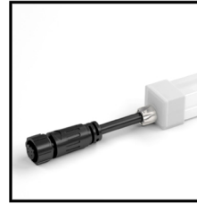
End Cap 5PIN Digital Order Code: 8921310-06 Color: white Cable entry: front/side/bottom Picture: front
