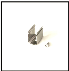
Mounting Clips Order Code: 8971212-03 Dimension: L30xW14xH14.5mm Material: stainless steel Color: silver Each meter led strips needs 2 clips + 2 screws
