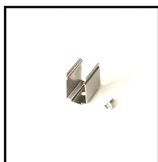
Mounting Clips Order Code: 8951616-03 Dimension: L20xW16.6xH12.4mm Material: stainless steel Color: silver Each meter led strips needs 2 clips + 2 screws
