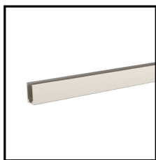
Aluminium Profile Order Code: 8951616-01 Dimension: L1000xW20.5xH17.6mm Material: aluminium Color: silver
