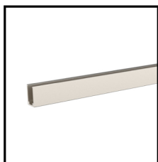
Aluminium Profile Order Code: 8951515-01 Dimension: L1000xW20.5xH17.6mm Material: aluminium Color: silver
